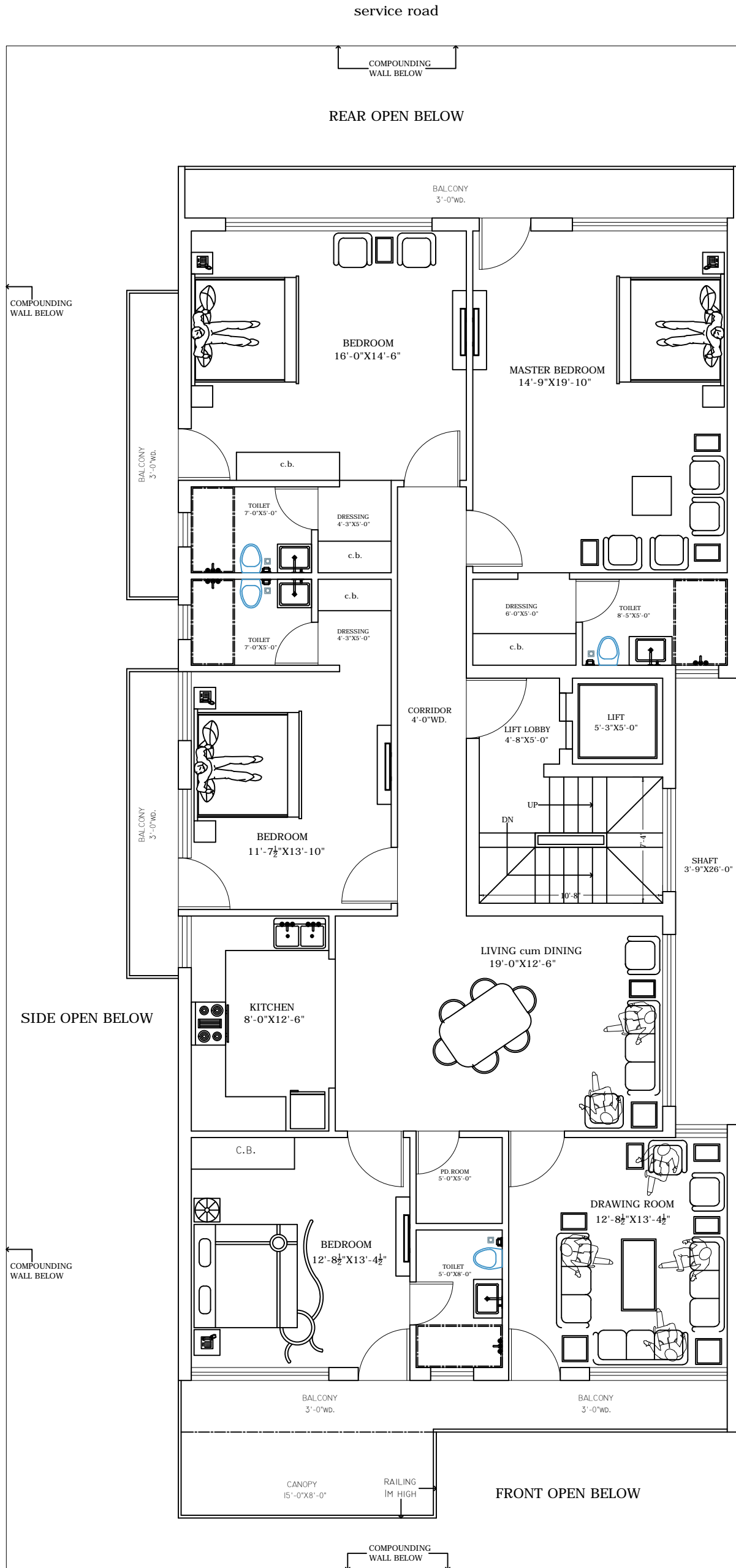
SKETCH LAY OUT PLAN OF TYPICAL FLOOR
